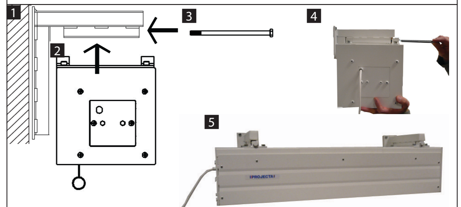
Mounting instruction
