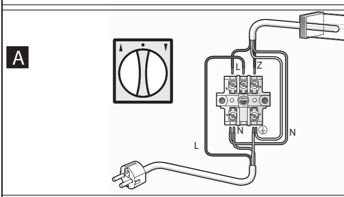
Mounting instruction
