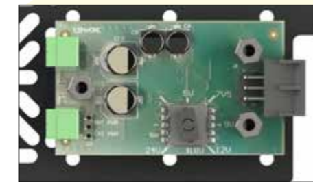
▲ Power circuit with voltage selector for a choice of 7 different voltages. Includes a pass thru option for custom power voltages supplied by 3rd party manufacturers
